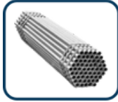
SCAFFOLD TUBE Diameter: 48.3mm Length: 0.5M TO 6.0M Standard: EN39/BS1139/EN10281
