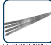
SCAFFOLD BOARD END-BAND Size: 546mmx 25mm Finish: HDG
